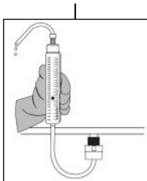
Figure 15. Check nozzle for uniform output with a quick nozzle flow tester. If nozzle are outside +/- 10% of the average output replace the nozzle.
