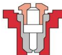
Figure 7. Pre-orifice flat-fan nozzles reduce the volume of driftable droplets.
