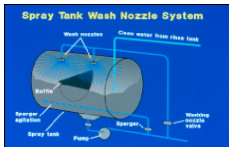
Figure 23. Correct tank mixing is essential for proper application.
