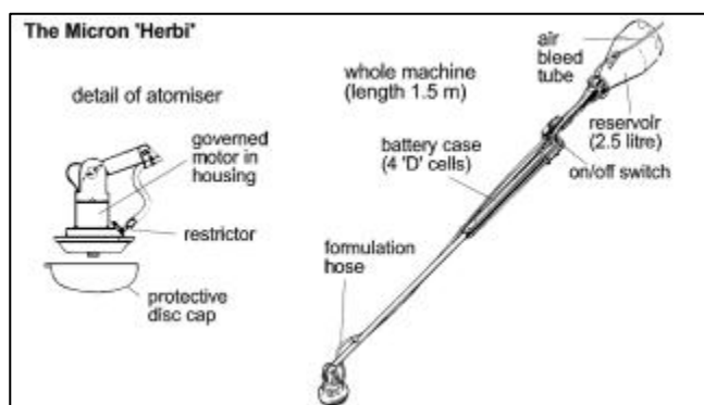
Figure 6. Controlled droplet applicators (CDA) configured in a handheld device.
