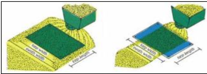
Figure 26. Collect output from a centrifugal applicator by operating the spreader over a tarp or plastic sheet of known dimensions. Then weigh the output.
