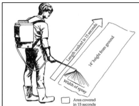
Figure 27. Determining coverage rate of a hand-held or hose-end sprayer.
