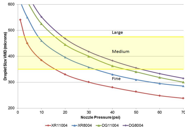
Figure 8. Comparing the mean droplet size of two extended range flat-fans (XR) with two pre-orifice flat-fans (DG).
