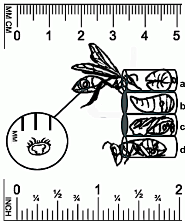
Figure 2. The Varroa mite life cycle occurs in conjunction with the honey bee reproductive cycle. The mother mite enters an uncapped brood cell via a nurse bee (a). She then begins to feed (b) and lays her eggs, which mature and mate (c). As the adult bee emerges, the mother mite and mated adult females exit on their host (d).
